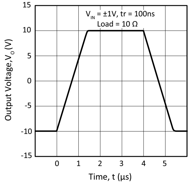
Figure 18: Loading Effects
