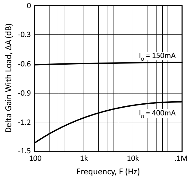
Figure 18: Loading Effects
