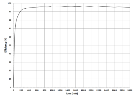
Fig 27: Electric Power Conversion Rate ( V_{OUT}=3.3V , FREQ=H, MODE=H)
